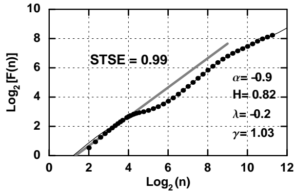
FIG. 6: DFA of a time series generated by the CBFM with the following parameters: b = 0.40 , a = 0.35 , \tau = 15 and \sigma = 0.20 .
